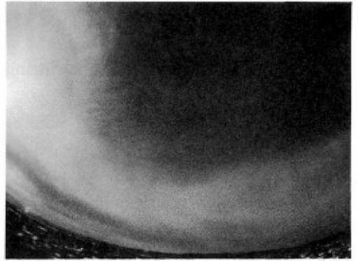
Fig. 3. This photograph shows the right hand 120-degree parhelia and a part of the parhelic circle.
